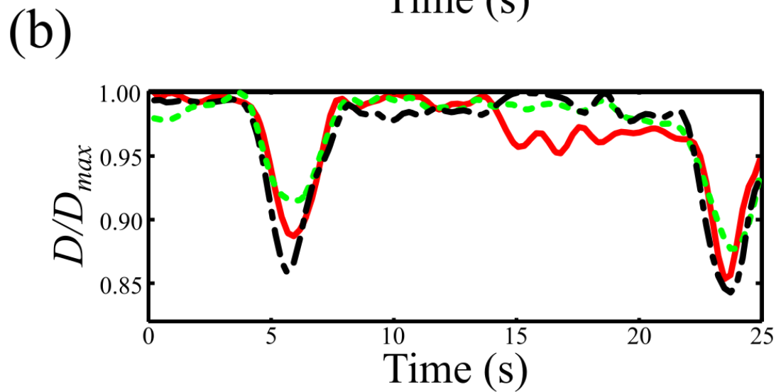
Figure 14: (a) Changes in vessel diameter ( D ) in WT Mouse at three segments for 25 seconds. Red (solid) curve depicts the segment downstream of the normal bi-leaflet valve, gray (dashed) and black (double-dashed) curves represent the segments at center of the lymphangions; (b) Changes in vessel diameter ( D ) in MV Mouse at three segments for 25 seconds. Red (solid) curve depicts the segment downstream of the bi-leaflet valve, green (dashed) curve depicts the segment downstream of the uni-leaflet valve and black (double-dashed) curve represents the segment at center of the lymphangion
